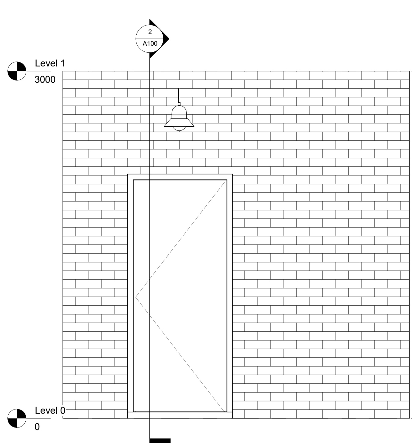
1 South - Graphic Display- Hidden Line 1 : 20
